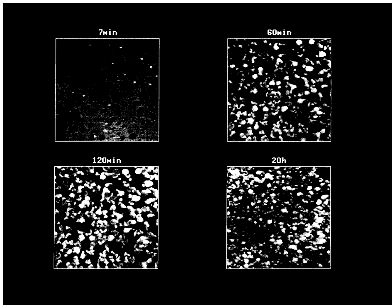
Fig. 3 5µm AFM topographies on the main surface of a 0.5 mm 30a -crystal upon exposure to air of 35% relative humidity at 22 °C at the times indicated; the z-scales are 100 nm in the first and 200 nm in the other images.
